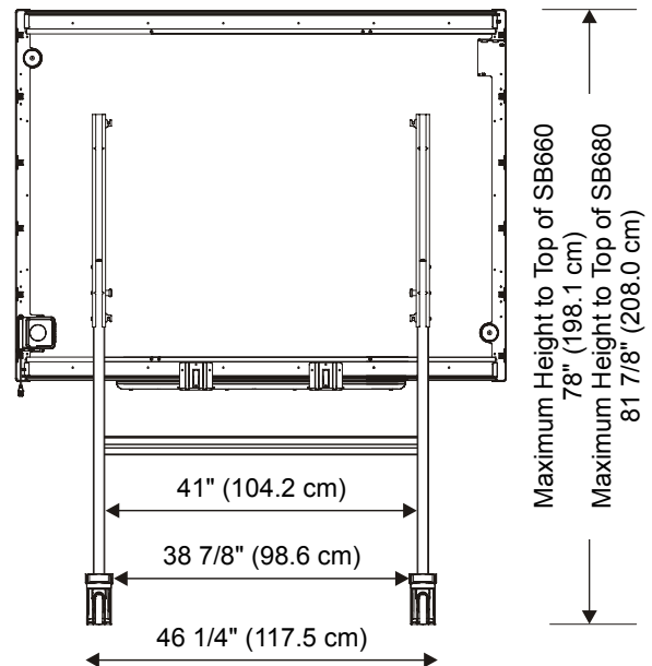
Floor Stand with SB680 Back View (highest position)
