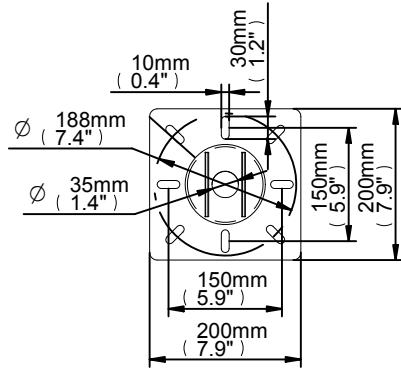
CEILING PLATE
