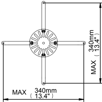
INTERFACE PLATE
